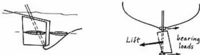
5-30. Lower bearing loads and better support with a skag.
