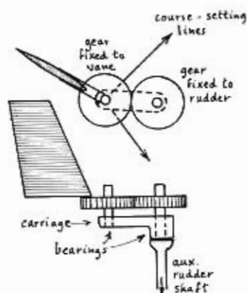
8-5. "Moving-carriage" vane.
