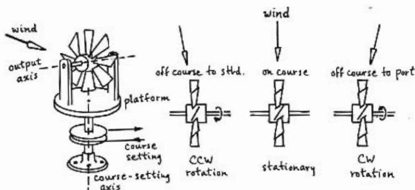
6-19. Windmill used as a wind-direction sensor.
