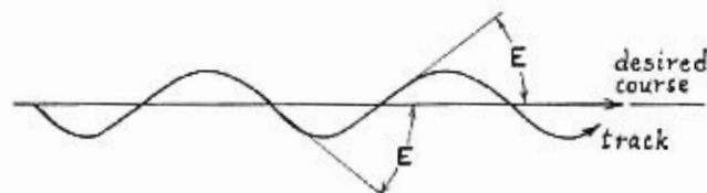
11-2. Oscillation adds half as much distance as a steady error in course.
