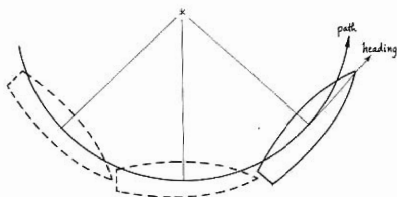
1-1 (b). Steady yaw without sideslip.
