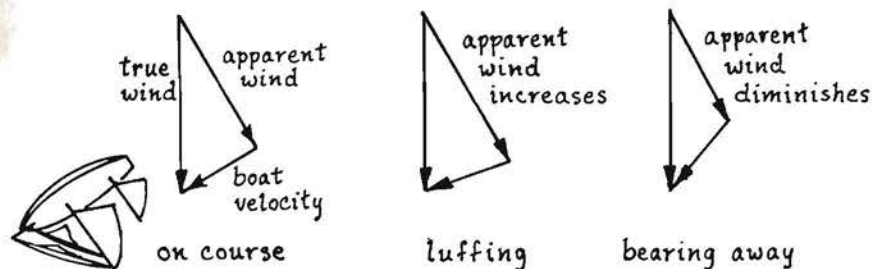
3-7. Strong variation of apparent wind with course changes on a beam reach.
