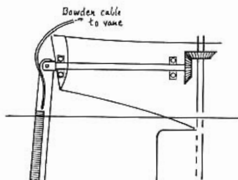
12-1. Built-in pendulum control.
